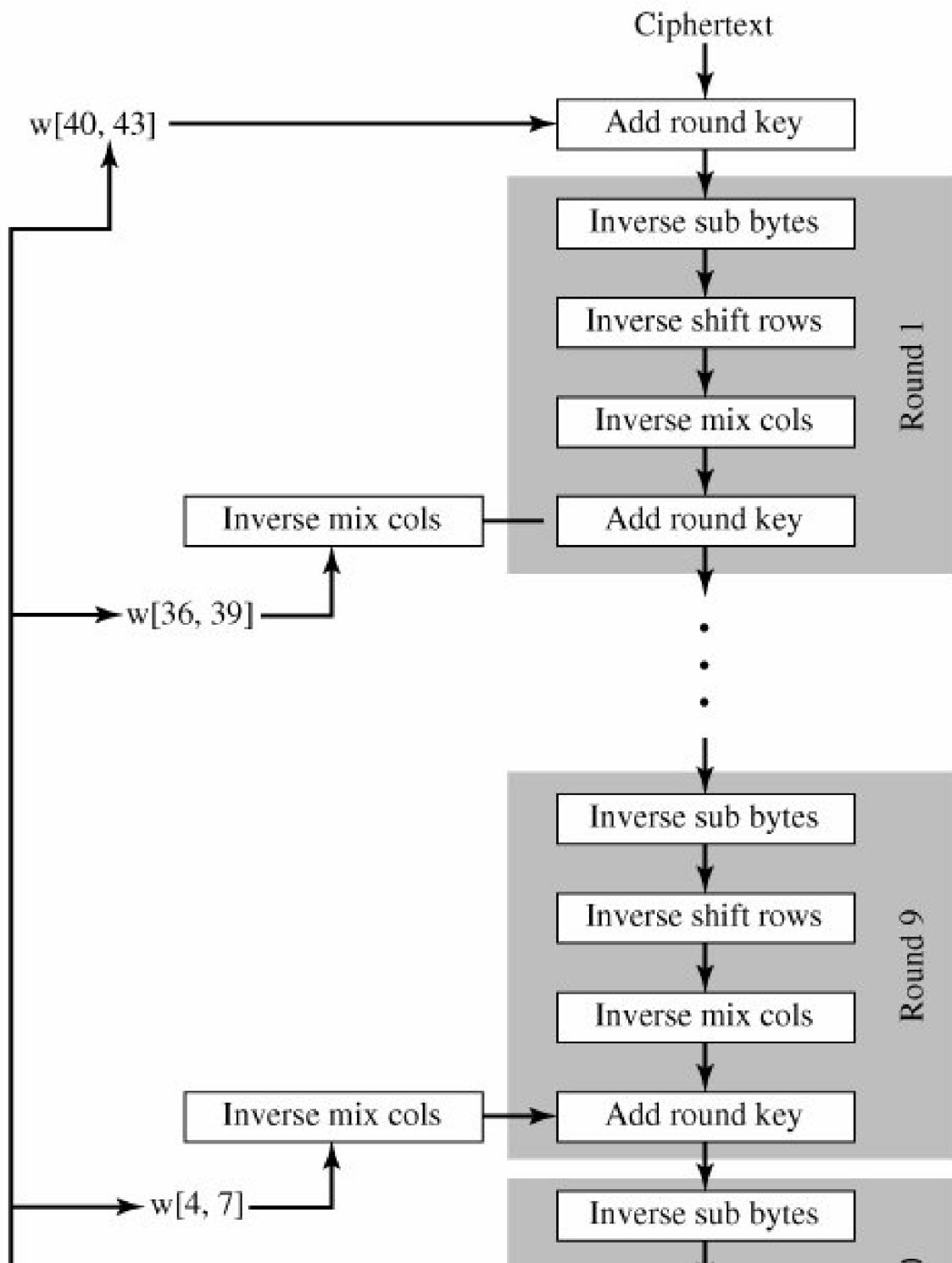
Figure 5.7. Equivalent Inverse Cipher (This item is displayed on page 158 in the print version)
