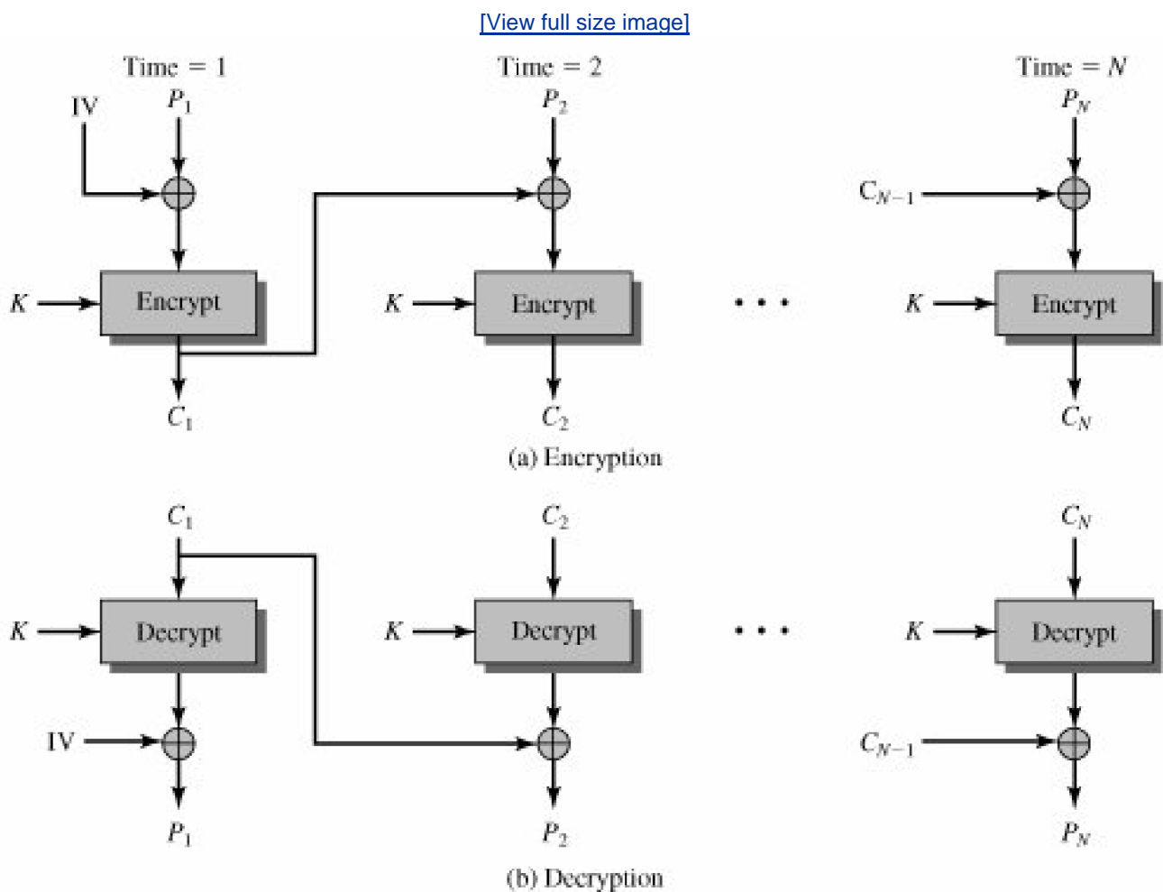
Figure 6.4. Cipher Block Chaining (CBC) Mode
