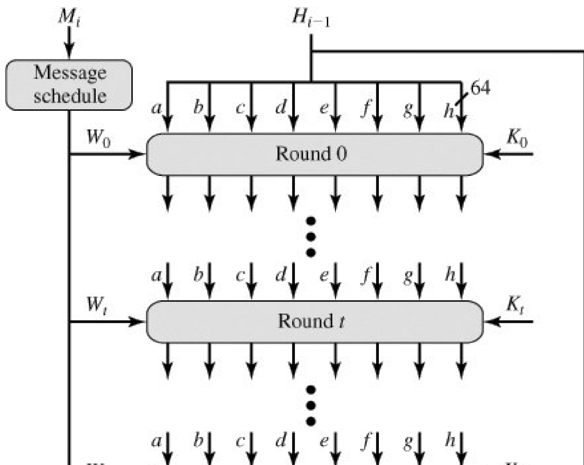
Figure 12.2. SHA-512 Processing of a Single 1024-Bit Block
