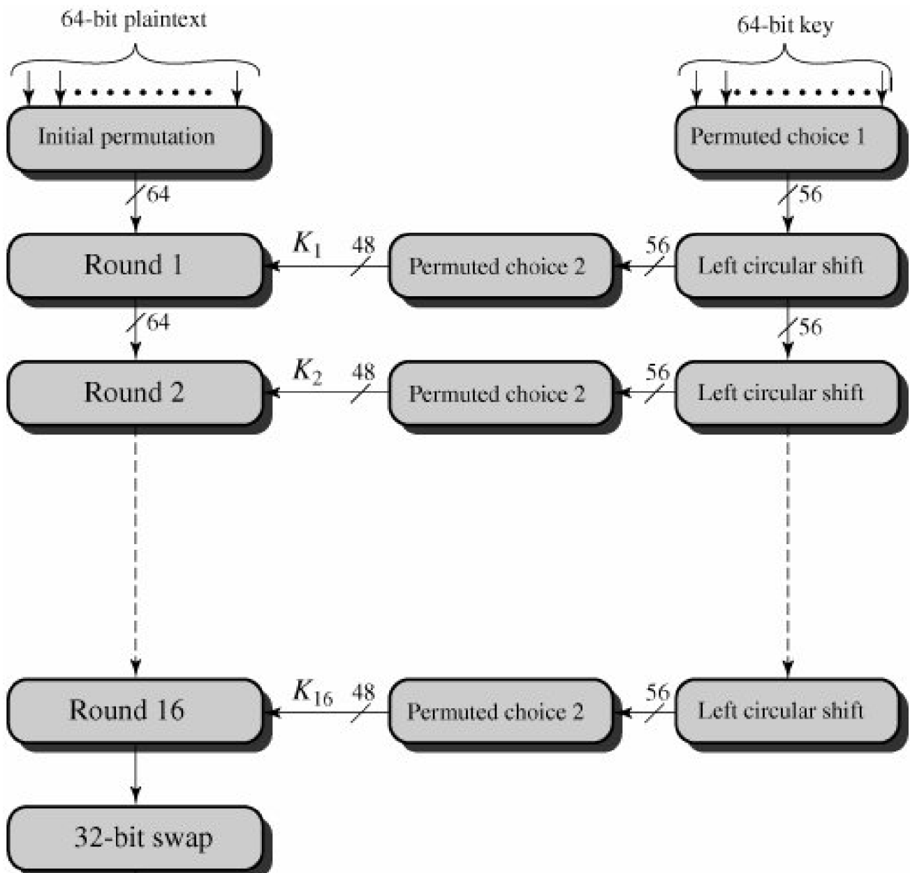
Figure 3.4. General Depiction of DES Encryption Algorithm
