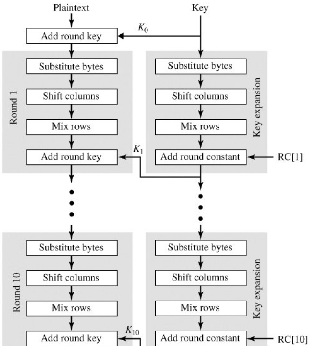
Figure 12.7. Whirlpool Cipher W
