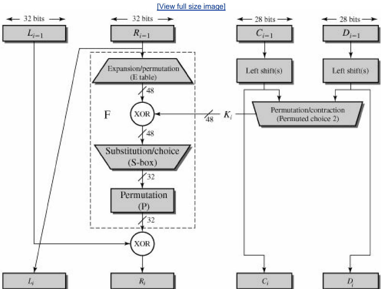
Figure 3.5. Single Round of DES Algorithm
