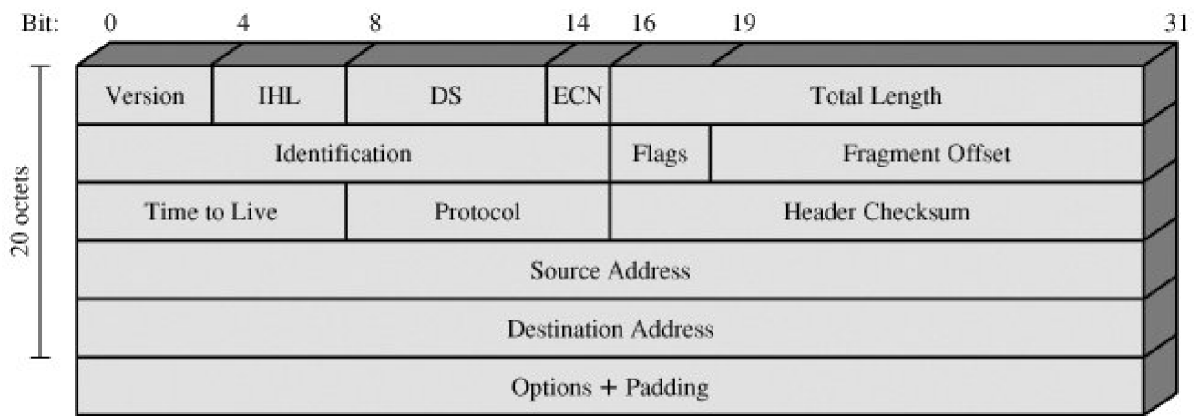
(a) IPv4 Header
