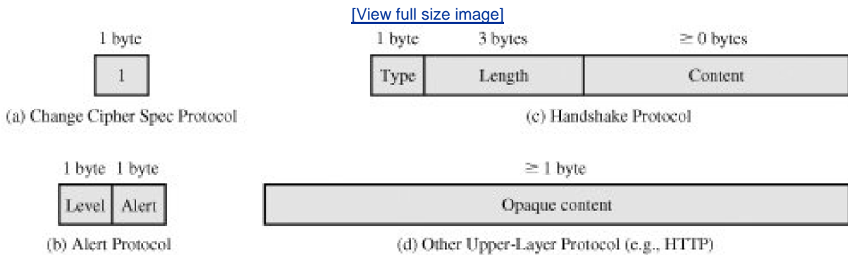
Figure 17.5. SSL Record Protocol Payload (This item is displayed on page 536 in the print version)
