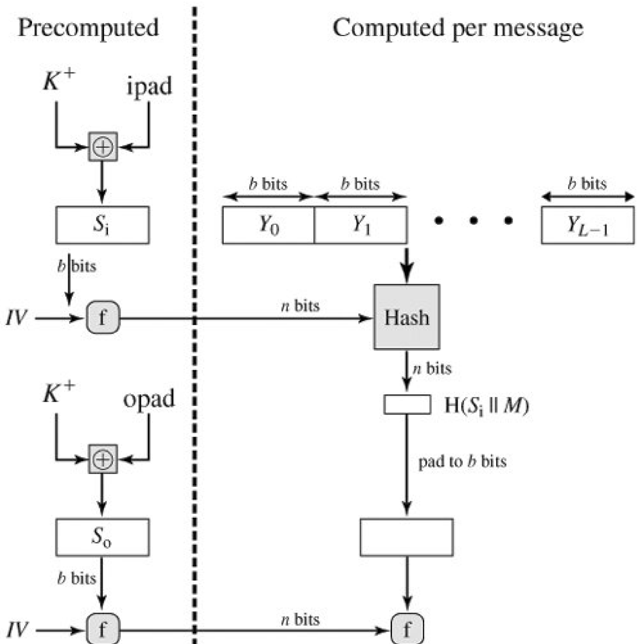
Figure 12.11. Efficient Implementation of HMAC (This item is displayed on page 371 in the print version)
