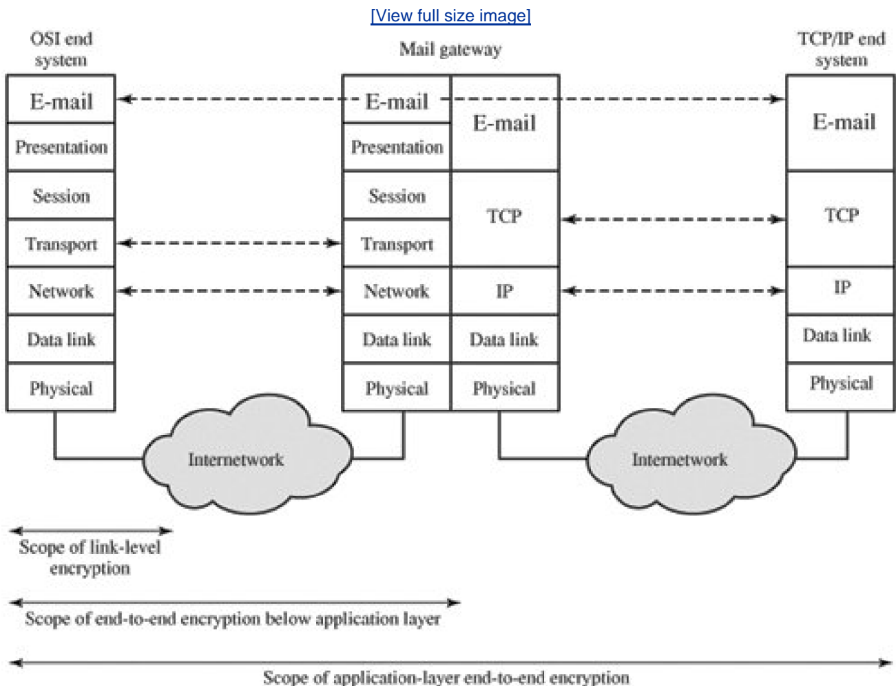
Figure 7.4. Encryption Coverage Implications of Store-and-Forward Communications
