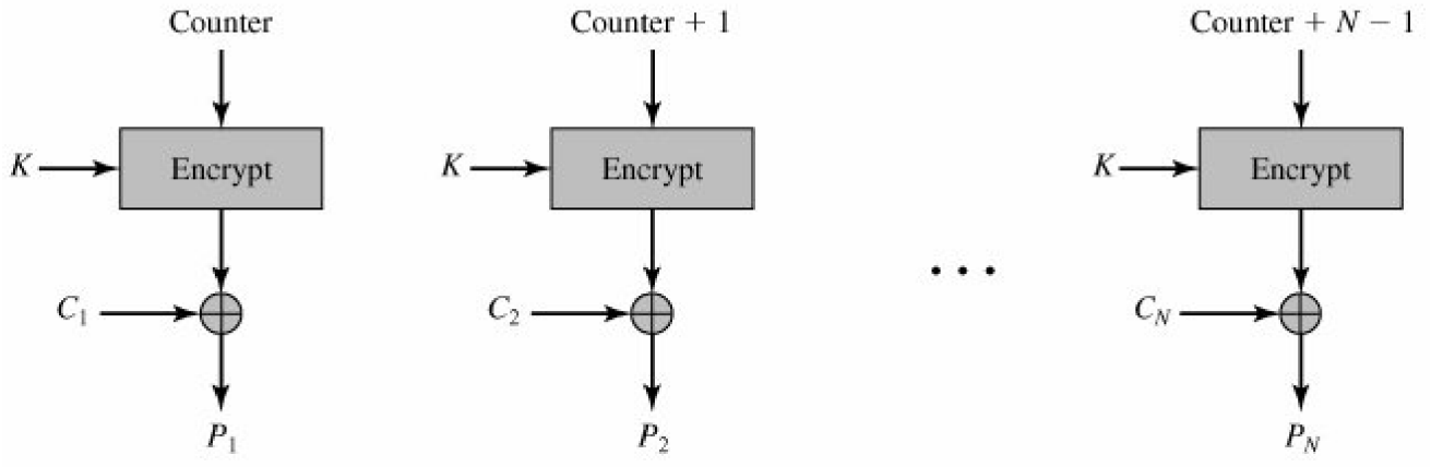
(b) Decryption
