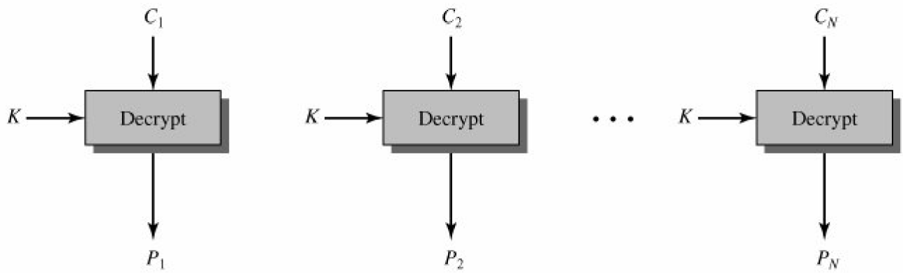
(b) Decryption
