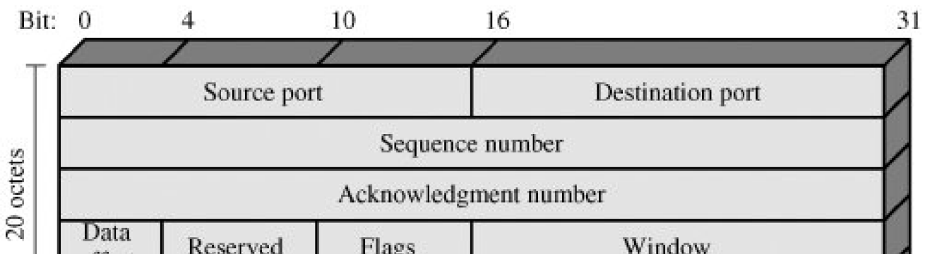
Figure 11.3. TCP Segment
