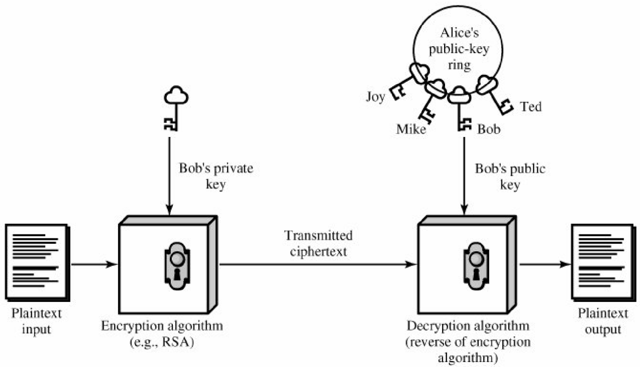
(b) Authentication
