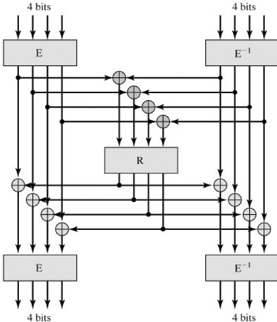
Figure 12.9. Implementation of Whirlpool S-Box (This item is displayed on page 366 in the print version)
