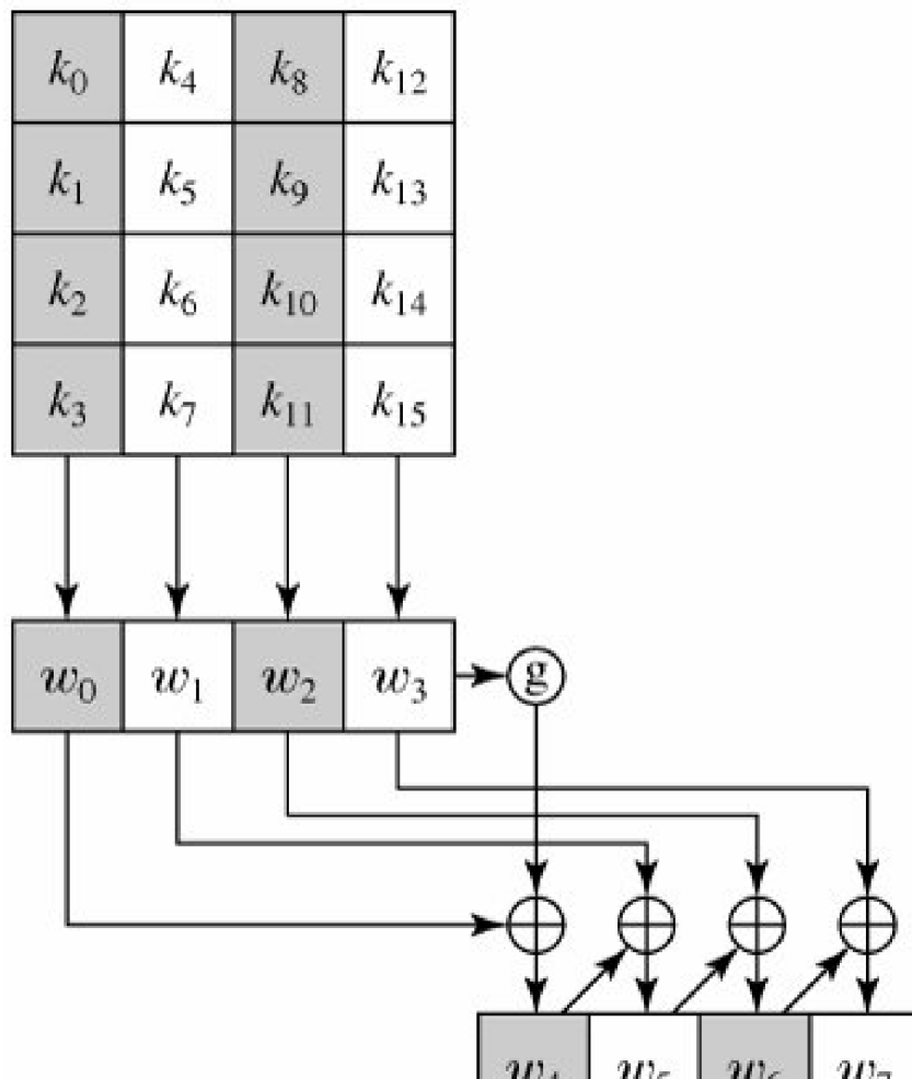
Figure 5.6. AES Key Expansion
