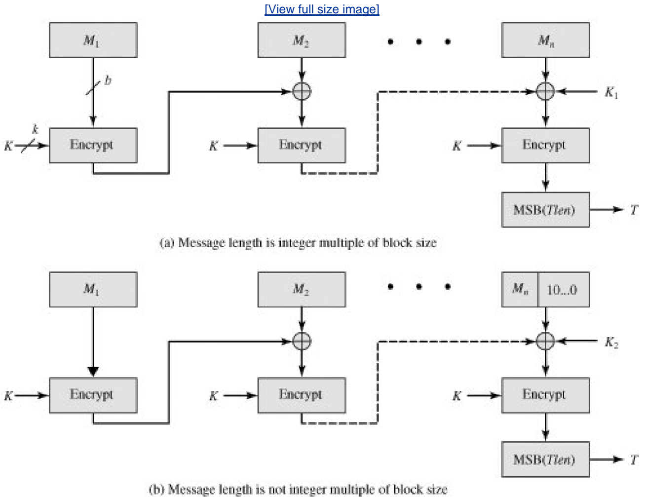
Figure 12.12. Cipher-Based Message Authentication Code (CMAC)
