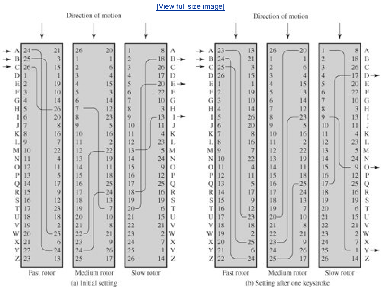
Figure 2.7. Three-Rotor Machine with Wiring Represented by Numbered Contacts (This item is displayed on page 52 in the print version)
