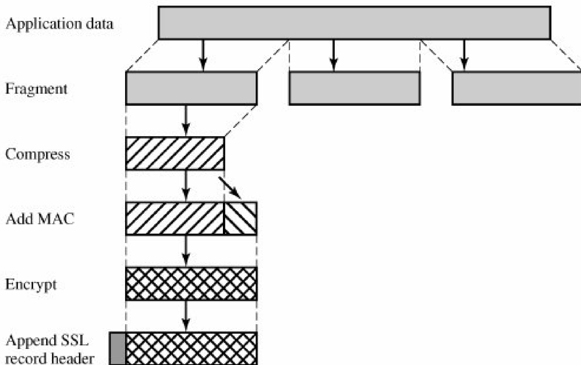
Figure 17.3. SSL Record Protocol Operation (This item is displayed on page 534 in the print version)
