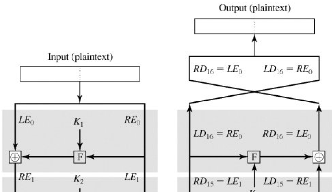
Figure 3.3. Feistel Encryption and Decryption (This item is displayed on page 71 in the print version)
