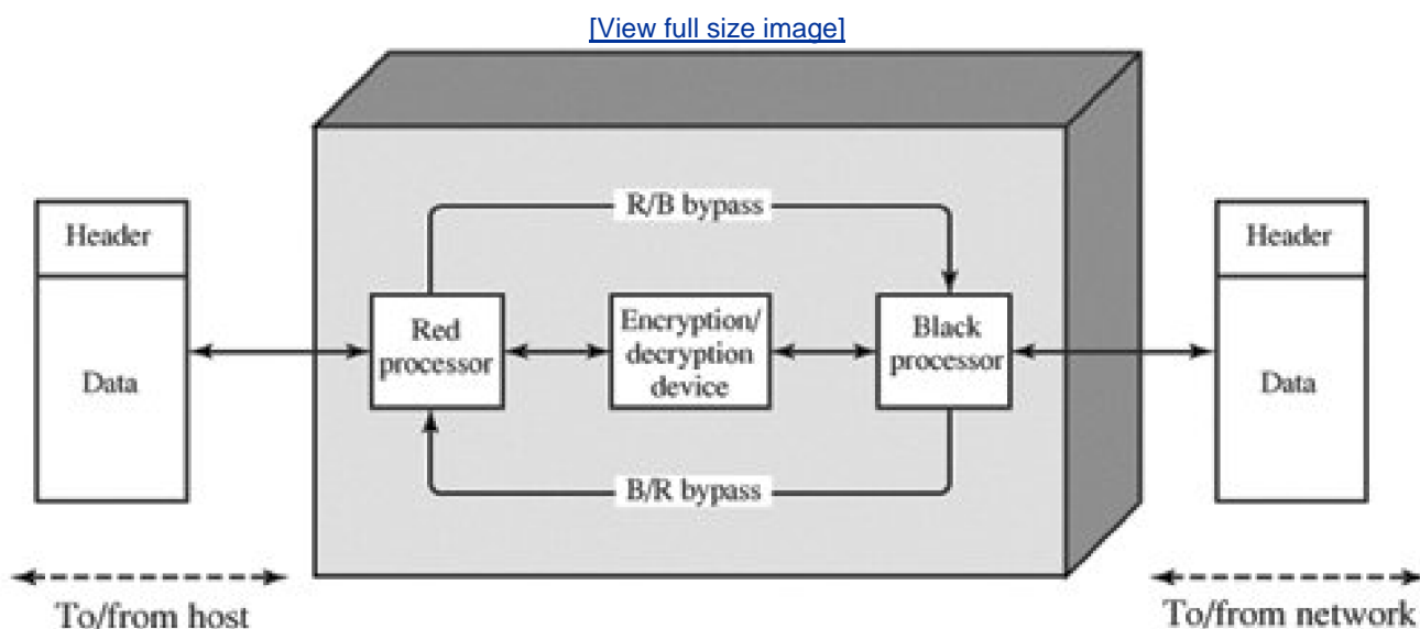
Figure 7.3. Front-End Processor Function
