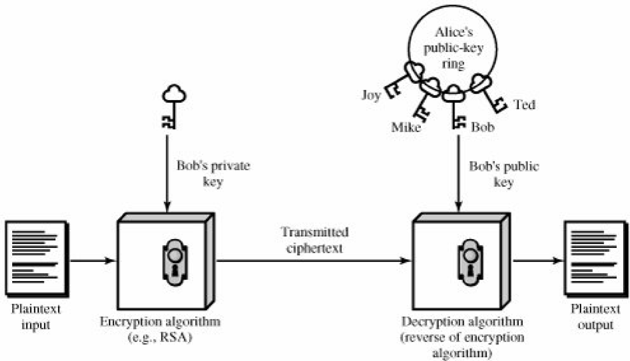
(b) Authentication
