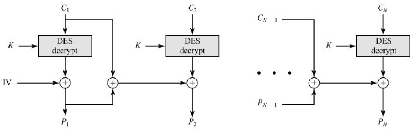
(b) Decryption
