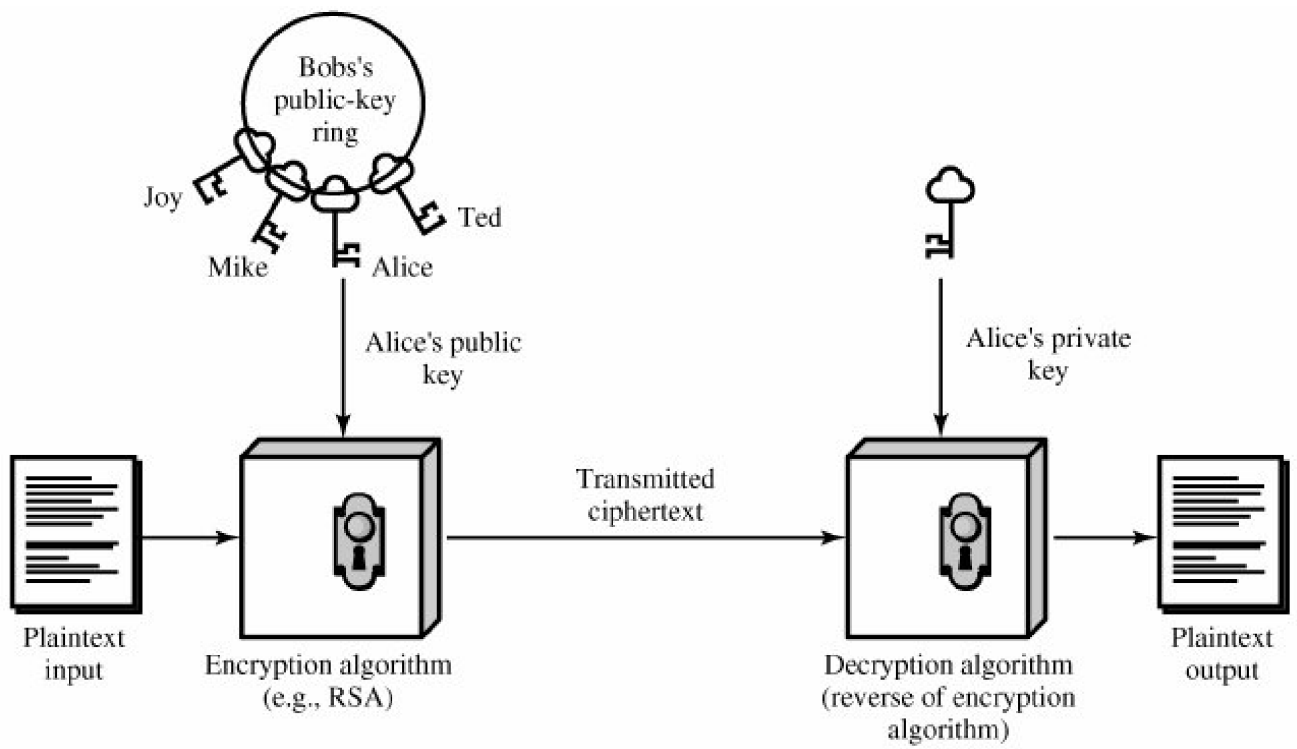
(a) Encryption
