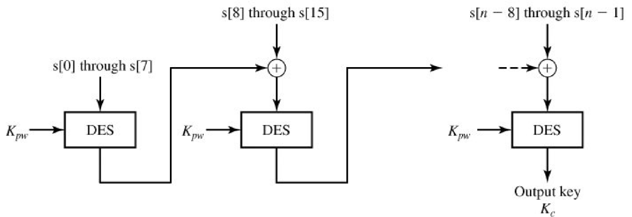
(c) Generate DES CBC checksum of password
