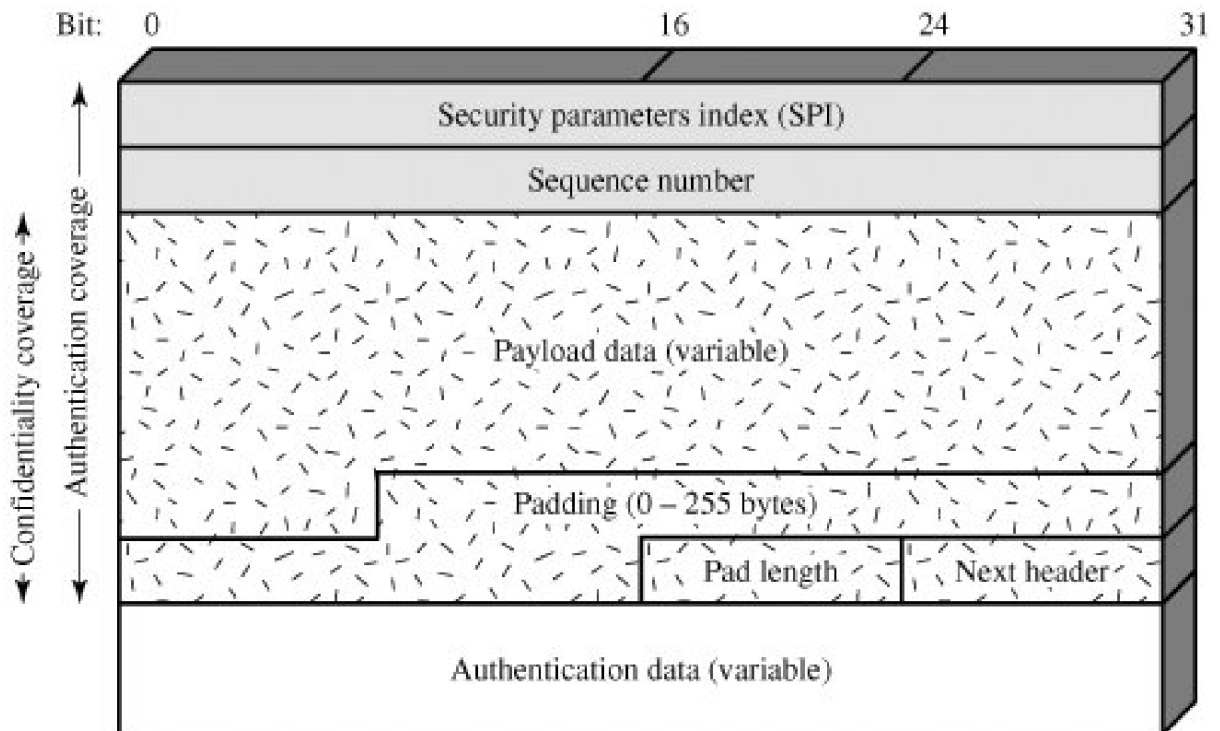
Figure 16.7. IPsec ESP format
