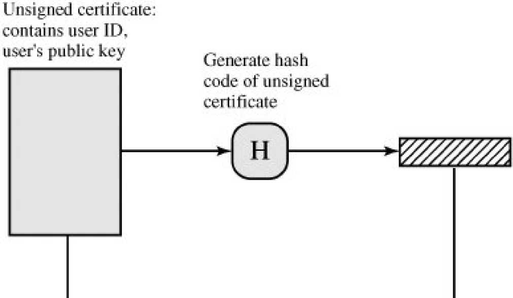
Figure 14.3. Public-Key Certificate Use
