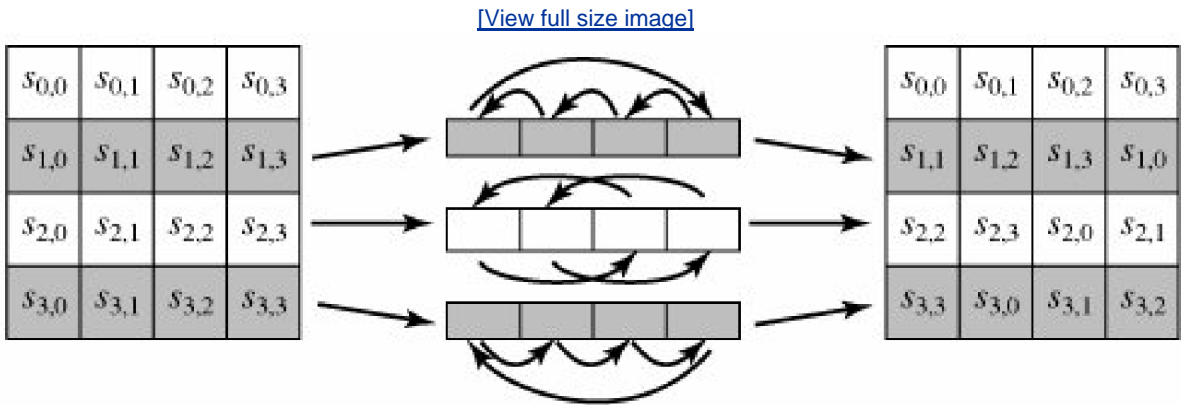
(a) Shift row transformation
