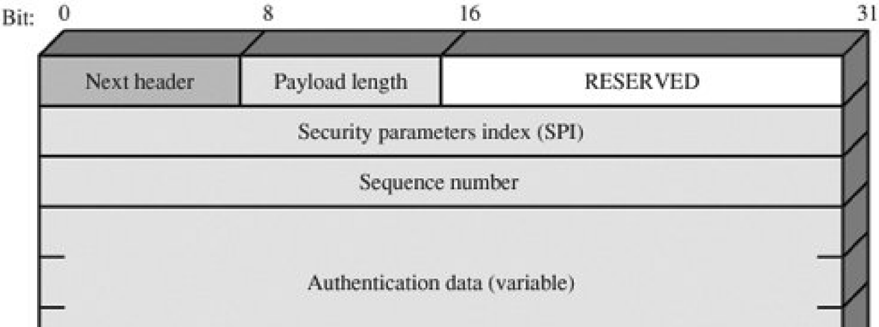
Figure 16.3. IPSec Authentication Header
