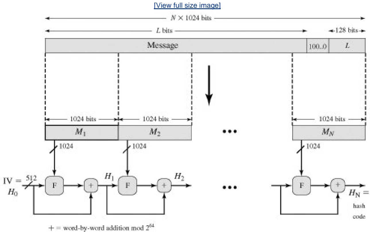
Figure 12.1. Message Digest Generation Using SHA-512
