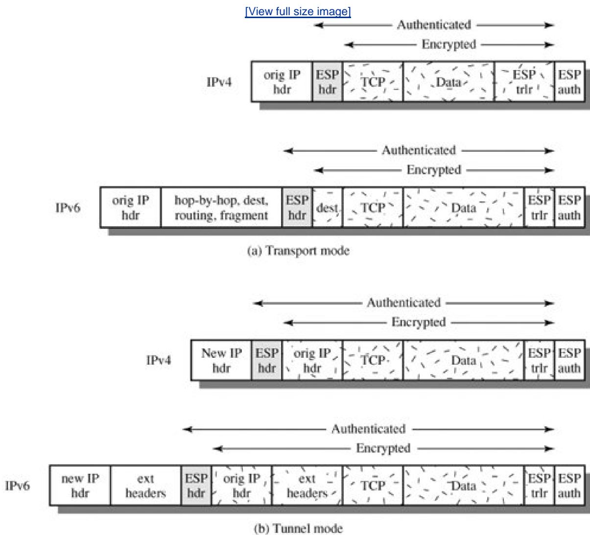
Figure 16.9. Scope of ESP Encryption and Authentication
