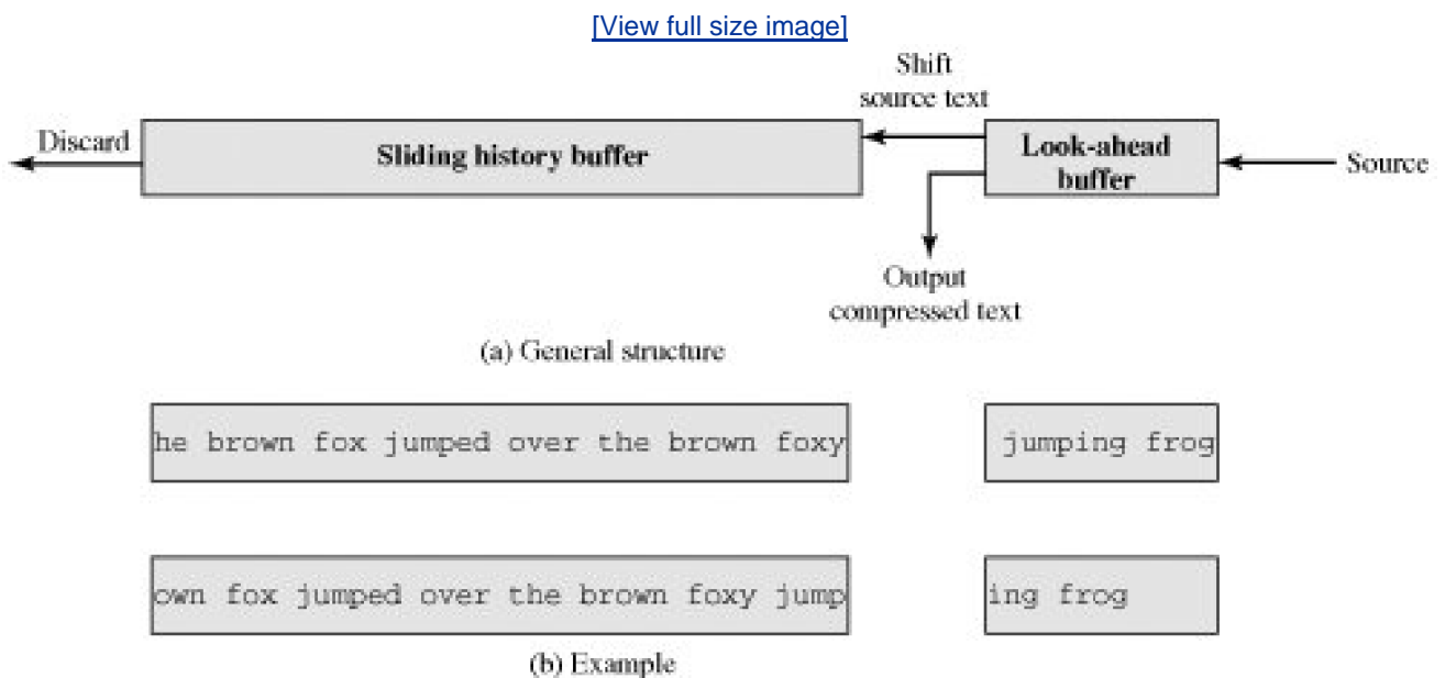
Figure 15.10. LZ77 Scheme
